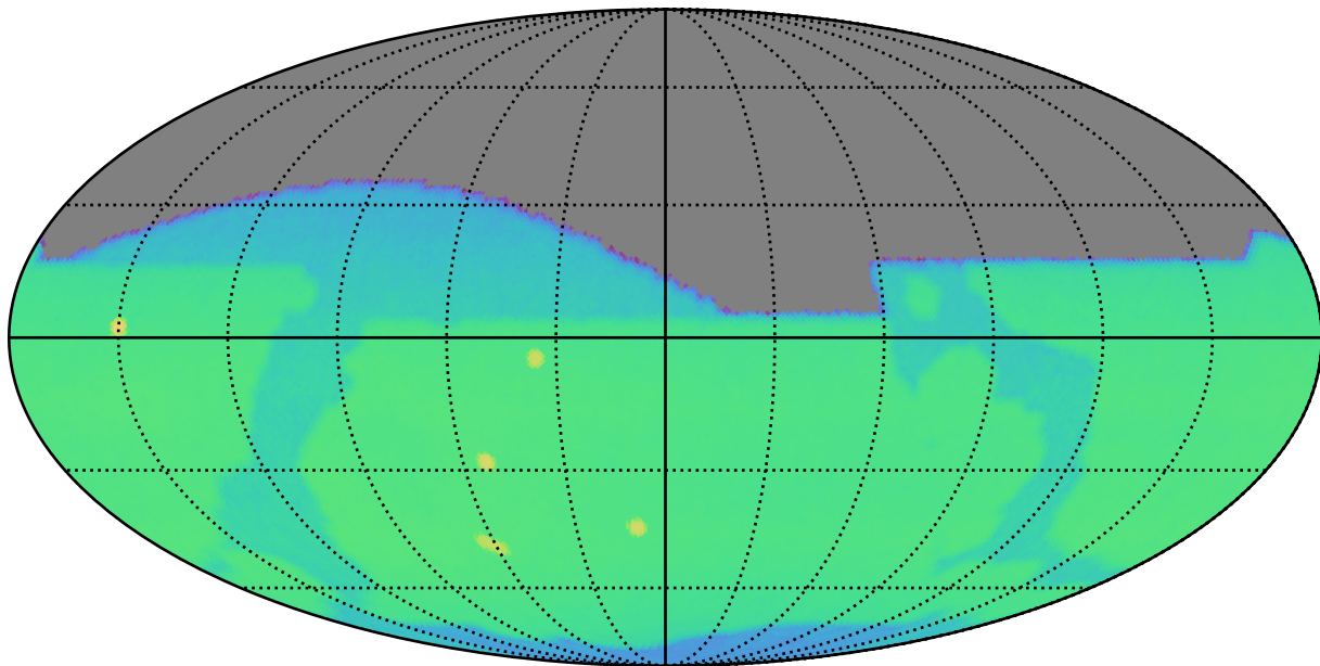
early_u_fpextra3.0_v3.4_10yrs i: CoaddM5
