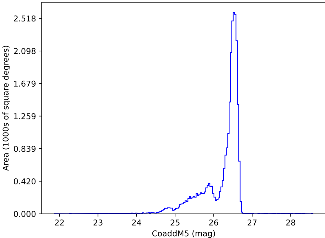
early_u_fpextra3.0_v3.4_10yrs i: CoaddM5
