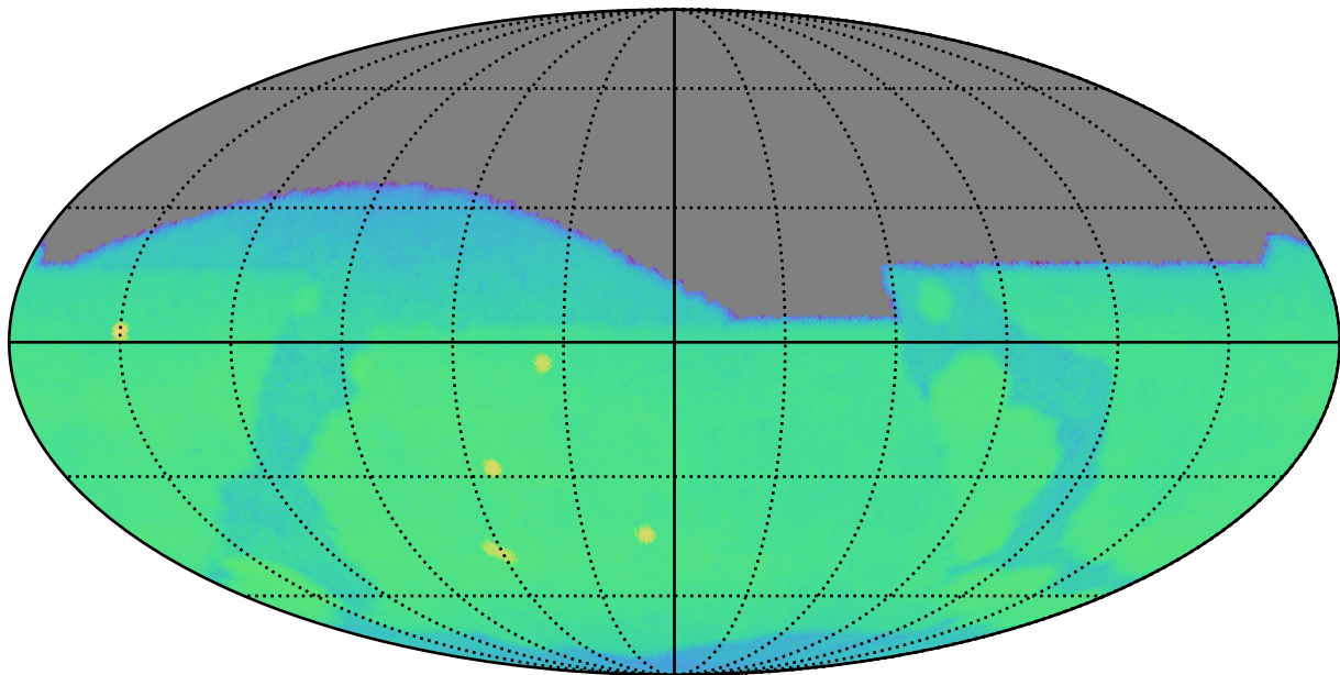
early_u_fpextra3.0_v3.4_10yrs g: CoaddM5
