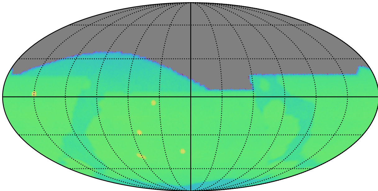
early_u_fpextra3.0_v3.4_10yrs : CoaddM5
