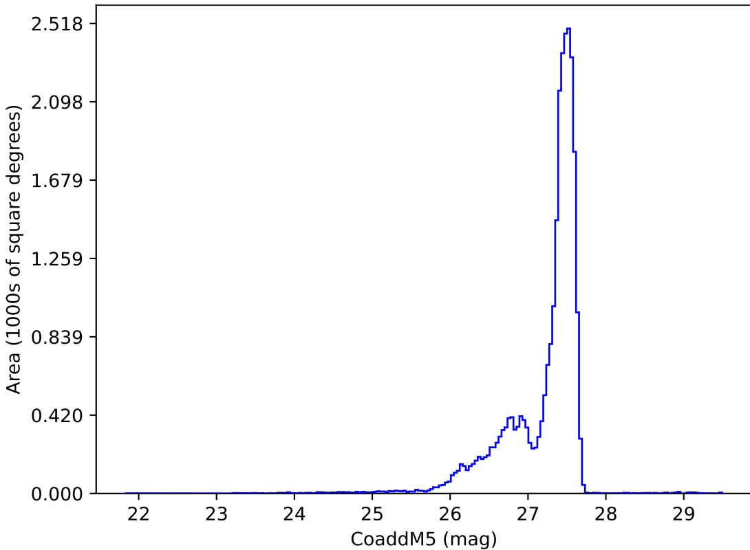
early_u_fpextra3.0_v3.4_10yrs : CoaddM5
