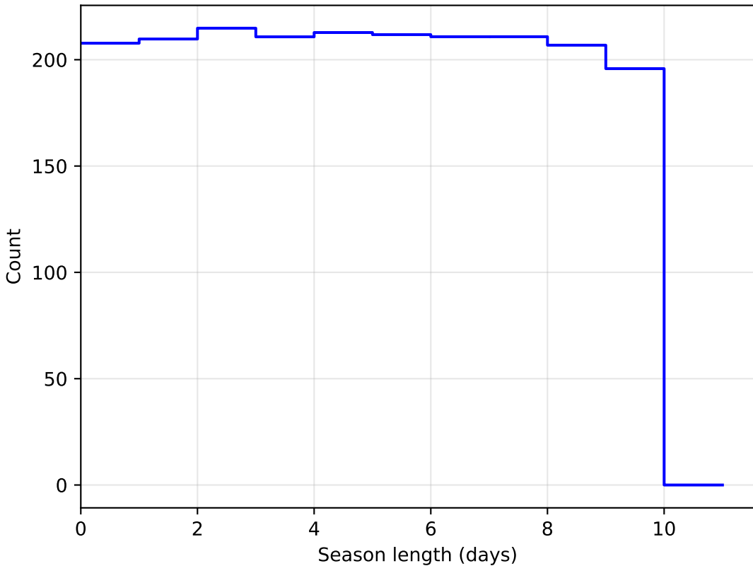
early_u_fpextra3.0_v3.4_10yrs DD:EDFS all bands: SeasonLength
