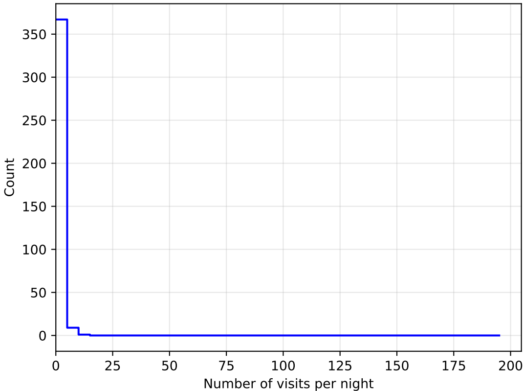
early_u_fpextra3.0_v3.4_10yrs all bands: DD:WFD NVisitsPerNight
