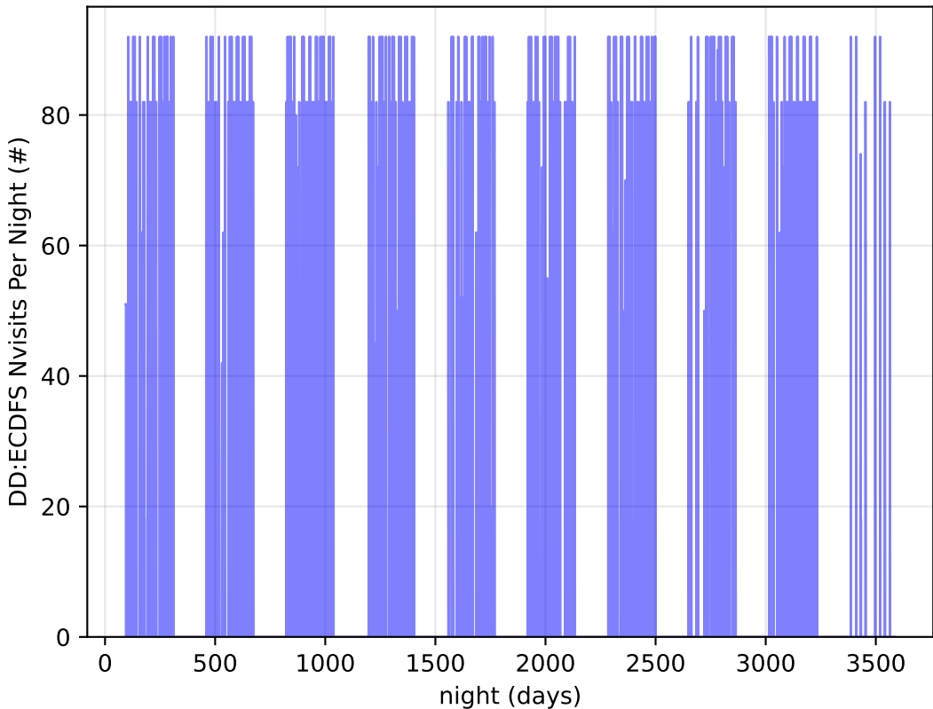
early_u_fpextra3.0_v3.4_10yrs all bands: DD:ECDFS Nvisits Per Night
