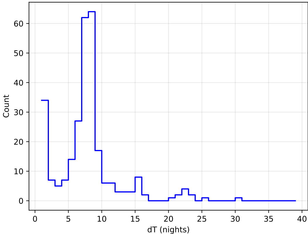
early_u_fpextra3.0_v3.4_10yrs all bands: DD:ECDFS Delta Nights Histogram
