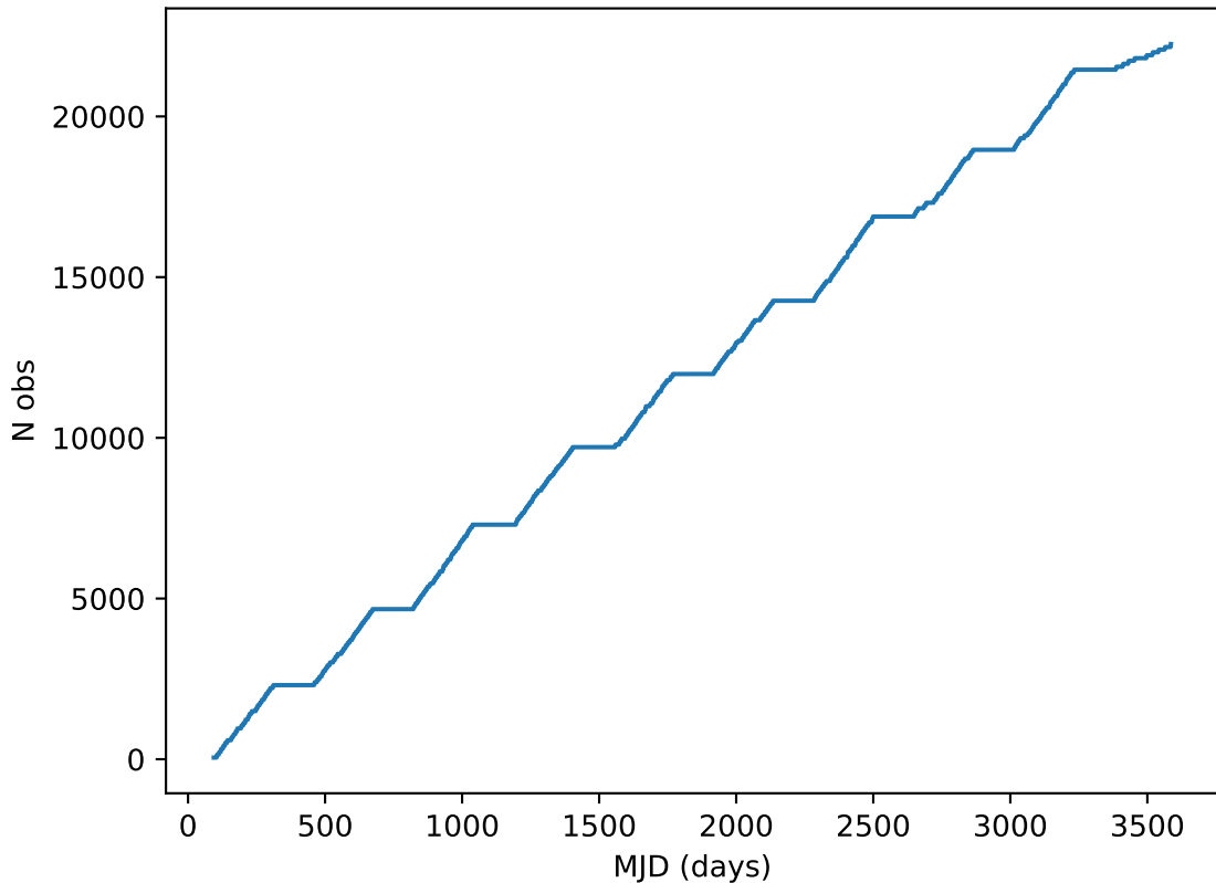
early_u_fpextra3.0_v3.4_10yrs all bands: DD:ECDFS Cumulative NVisits
