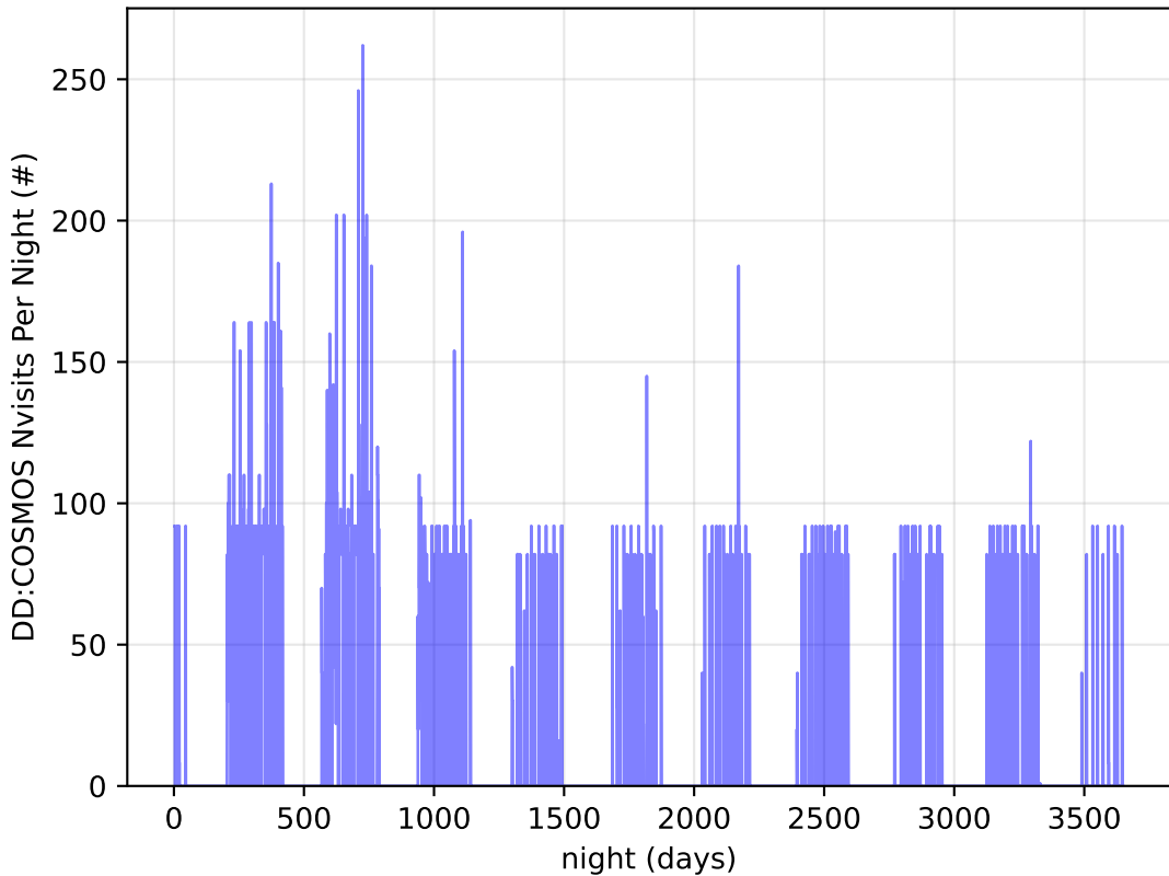
early_u_fpextra3.0_v3.4_10yrs all bands: DD: COSMOS Nvisits Per Night
