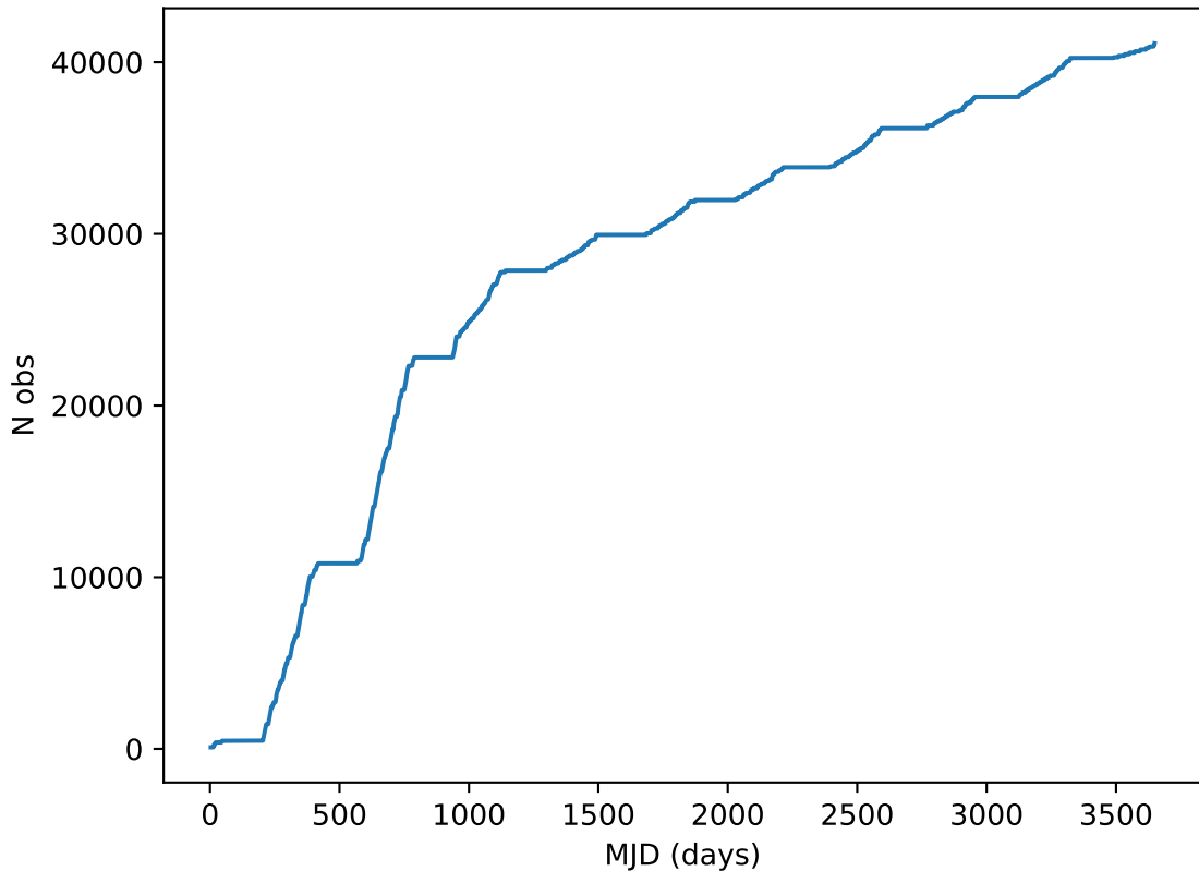
early_u_fpextra3.0_v3.4_10yrs all bands: DD: COSMOS Cumulative NVisits
