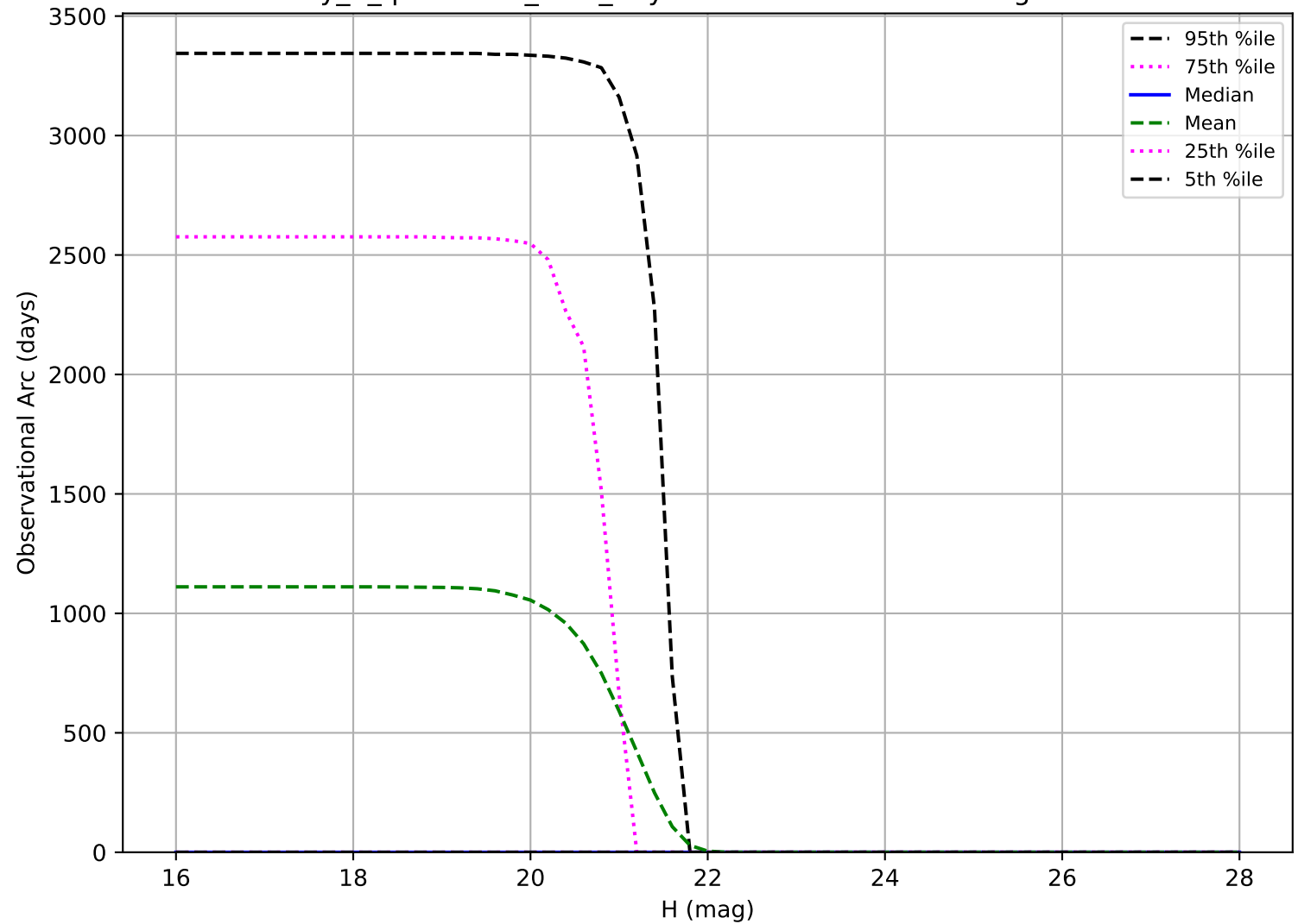
early_u_fpextra2.0_v3.4_10yrs: Observational Arc Length Vatra
