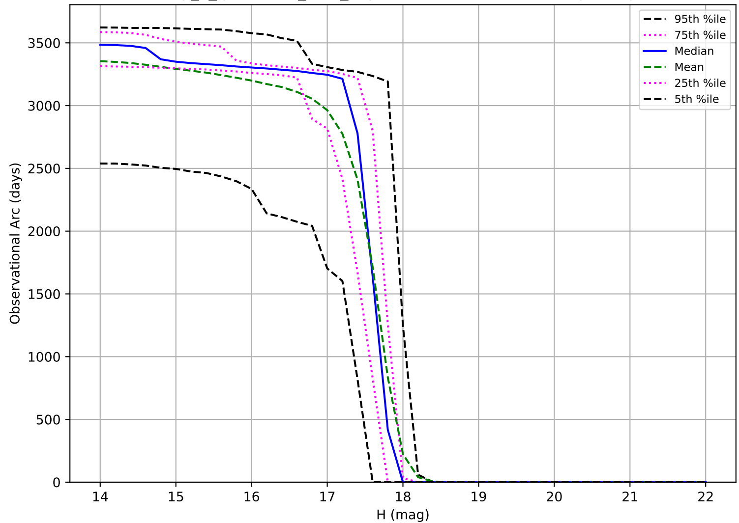
early_u_fpextra2.0_v3.4_10yrs: Observational Arc Length Trojan
