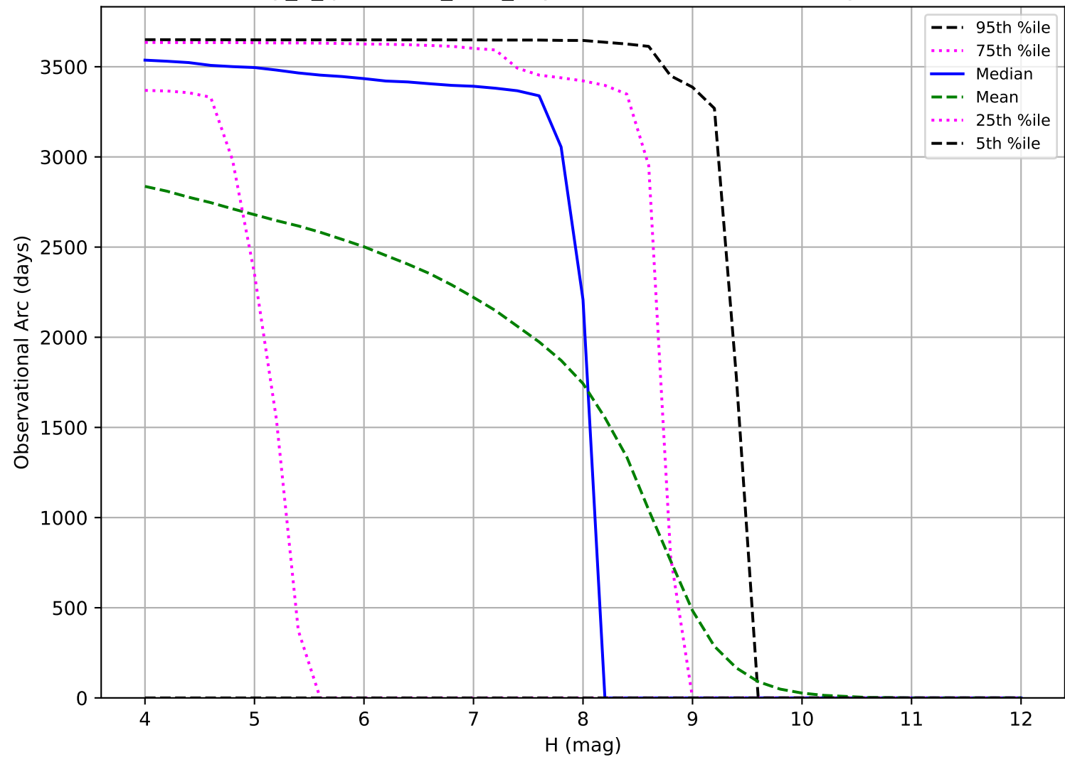
early_u_fpextra2.0_v3.4_10yrs: Observational Arc Length TNO
