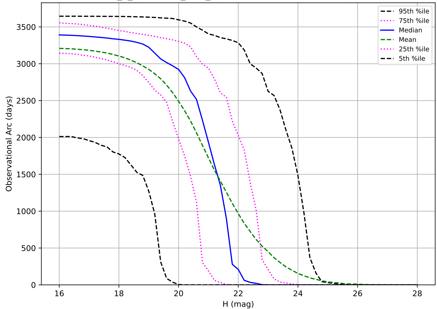
early_u_fpextra2.0_v3.4_10yrs: Observational Arc Length PHA
