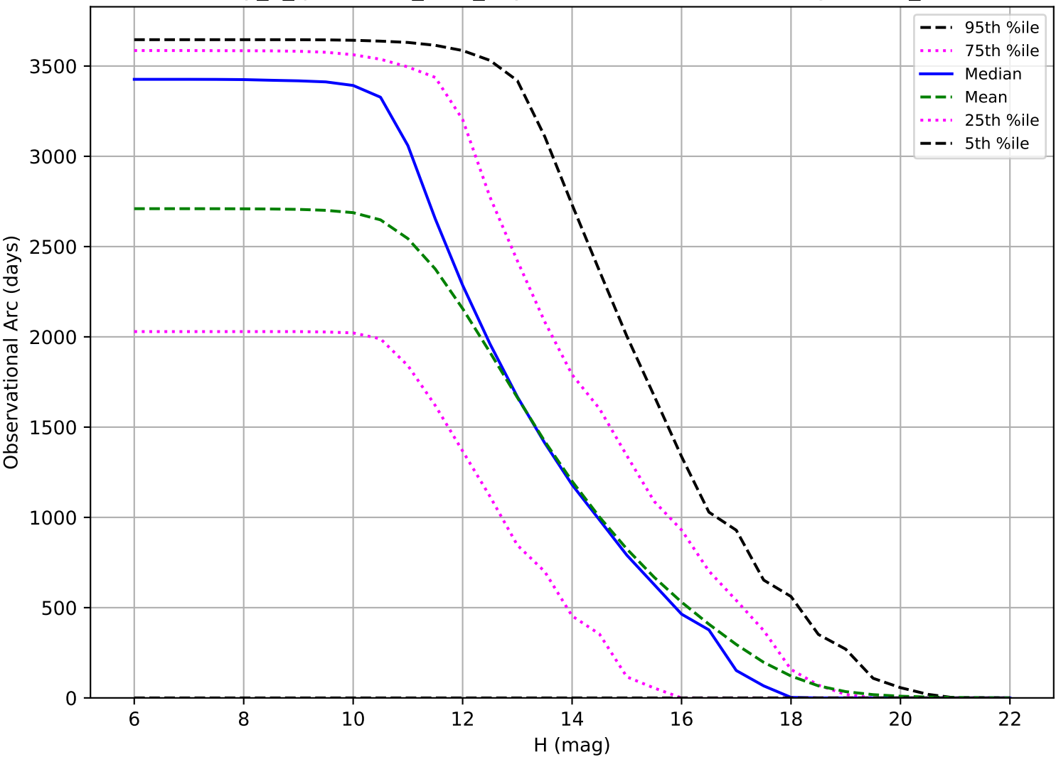
early_u_fpextra2.0_v3.4_10yrs: Observational Arc Length OCC_r5
