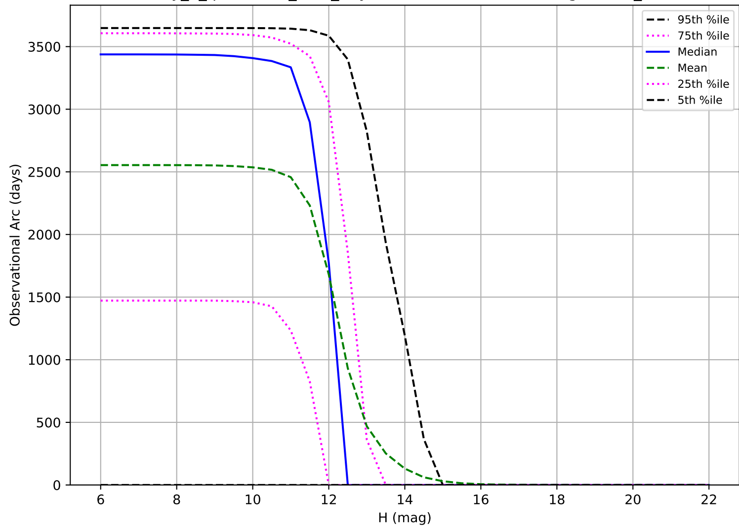
early_u_fpextra2.0_v3.4_10yrs: Observational Arc Length OCC_r20
