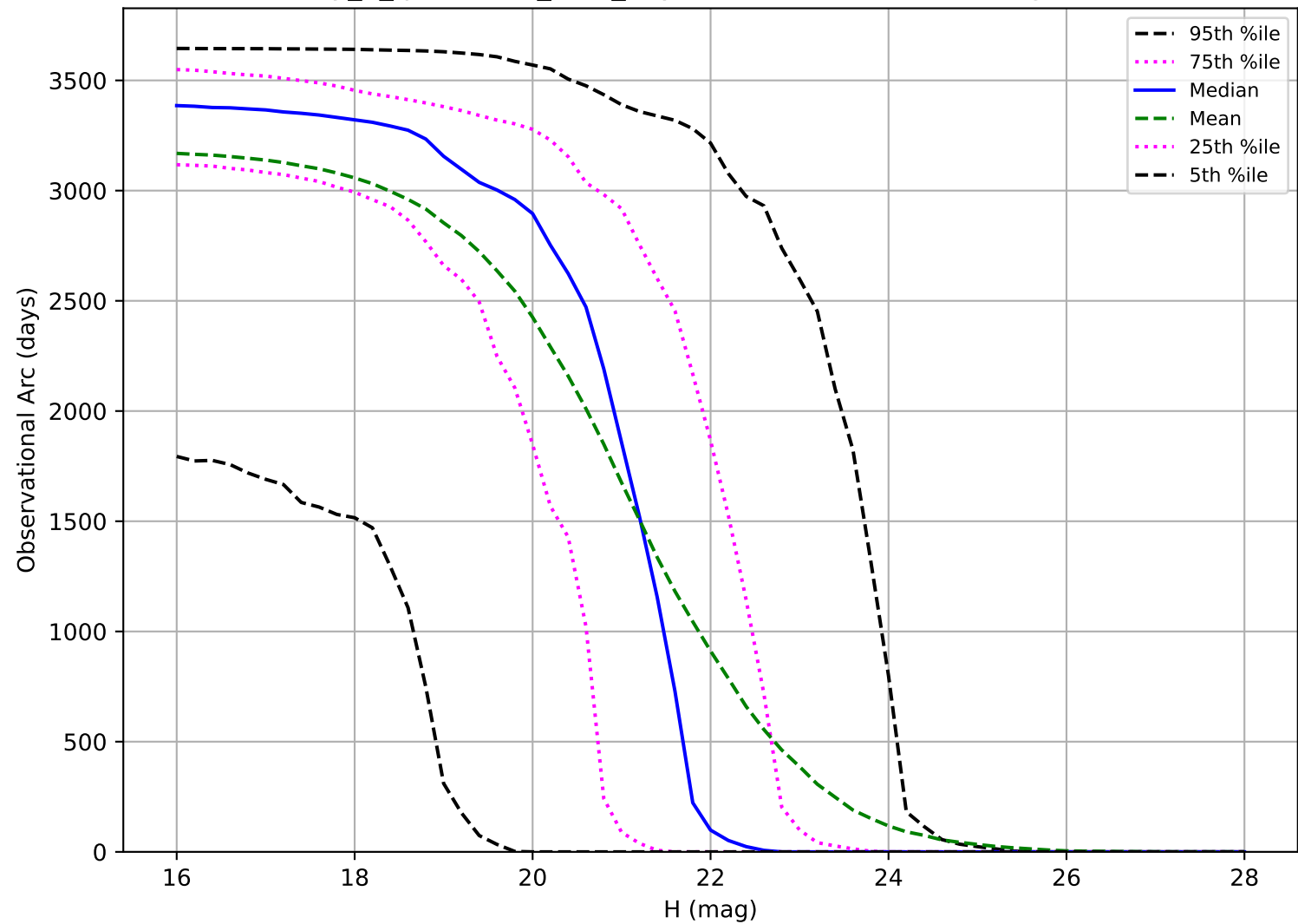
early_u_fpextra2.0_v3.4_10yrs: Observational Arc Length NEO
