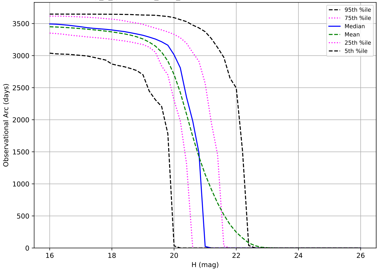
early_u_fpextra2.0_v3.4_10yrs: Observational Arc Length MBA
