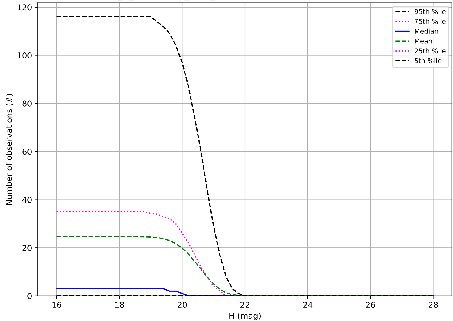
early_u_fpextra2.0_v3.4_10yrs: Number of observations Vatira
