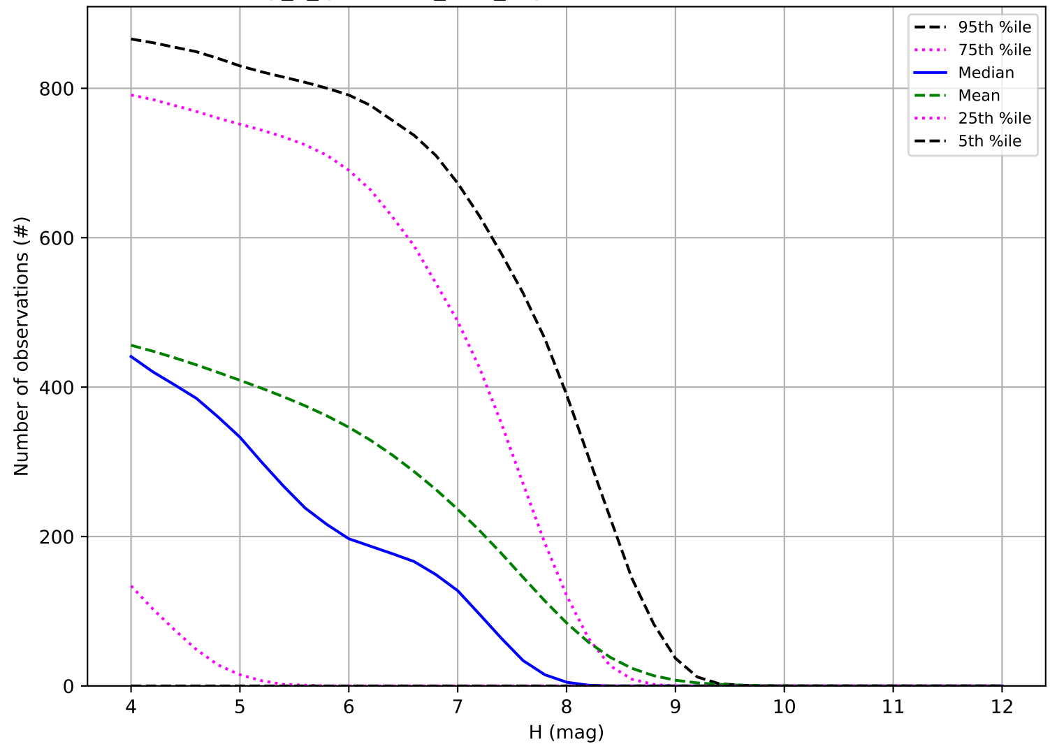
early_u_fpextra2.0_v3.4_10yrs: Number of observations TNO
