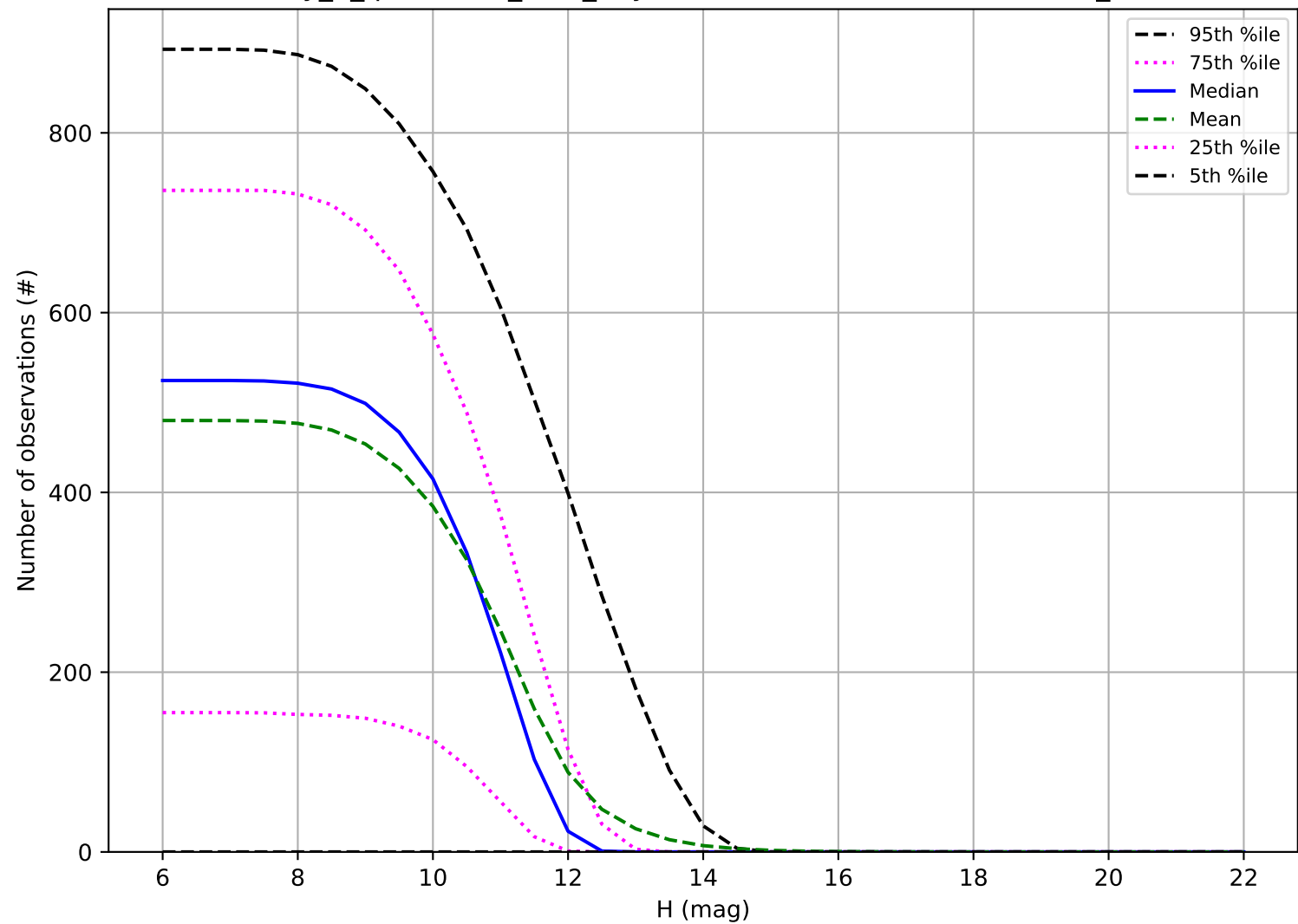
early_u_fpextra2.0_v3.4_10yrs: Number of observations OCC_r20
