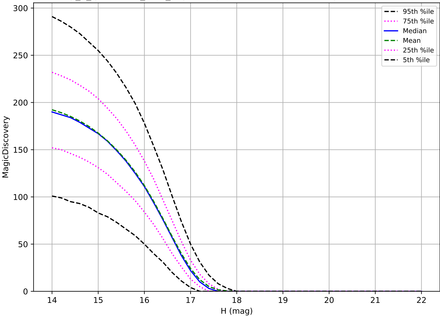
early_u_fpextra2.0_v3.4_10yrs: Trojan 6 detections in 60 nights detection loss
