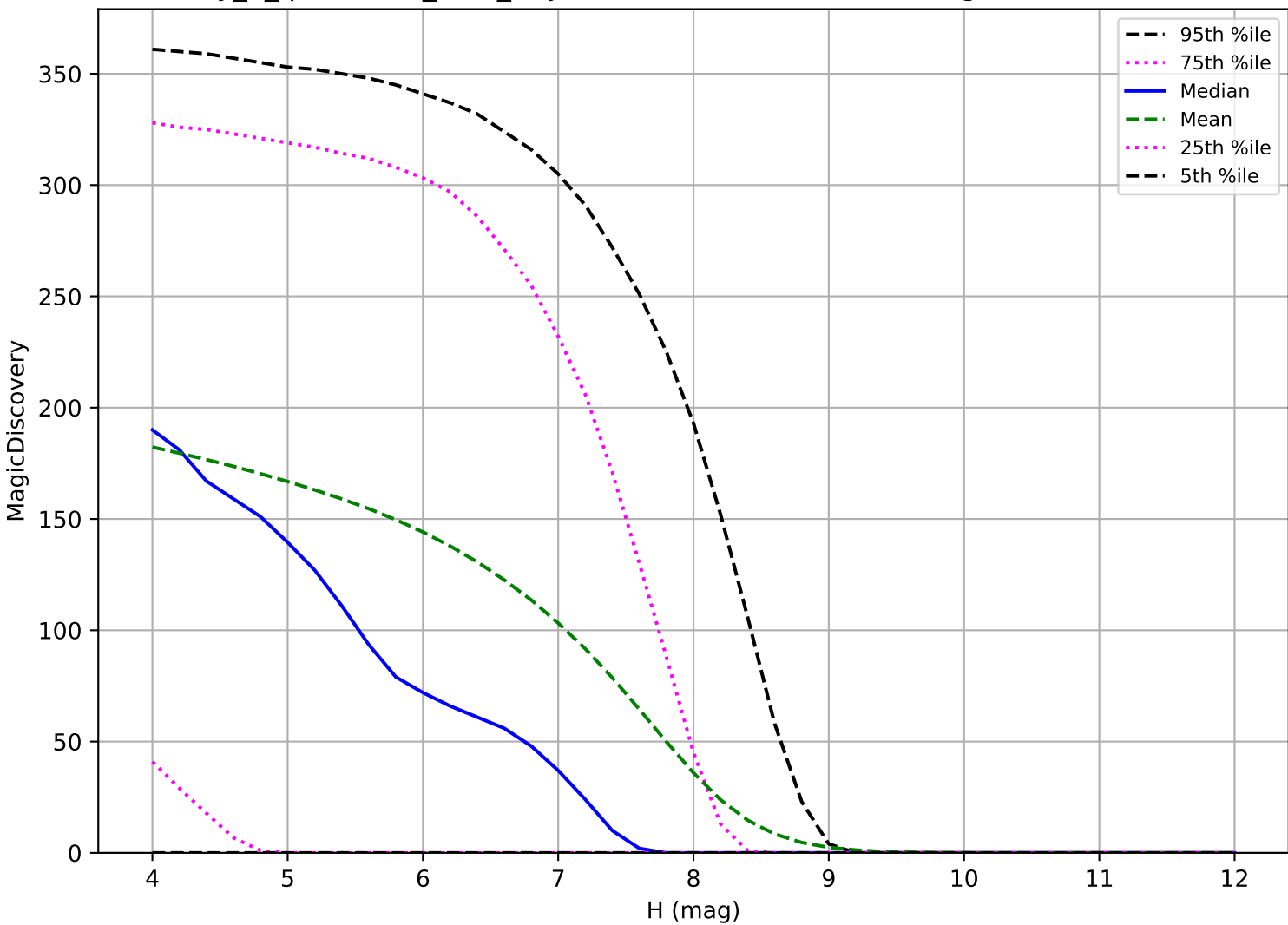
early_u_fpextra2.0_v3.4_10yrs: TNO 6 detections in 60 nights detection loss
