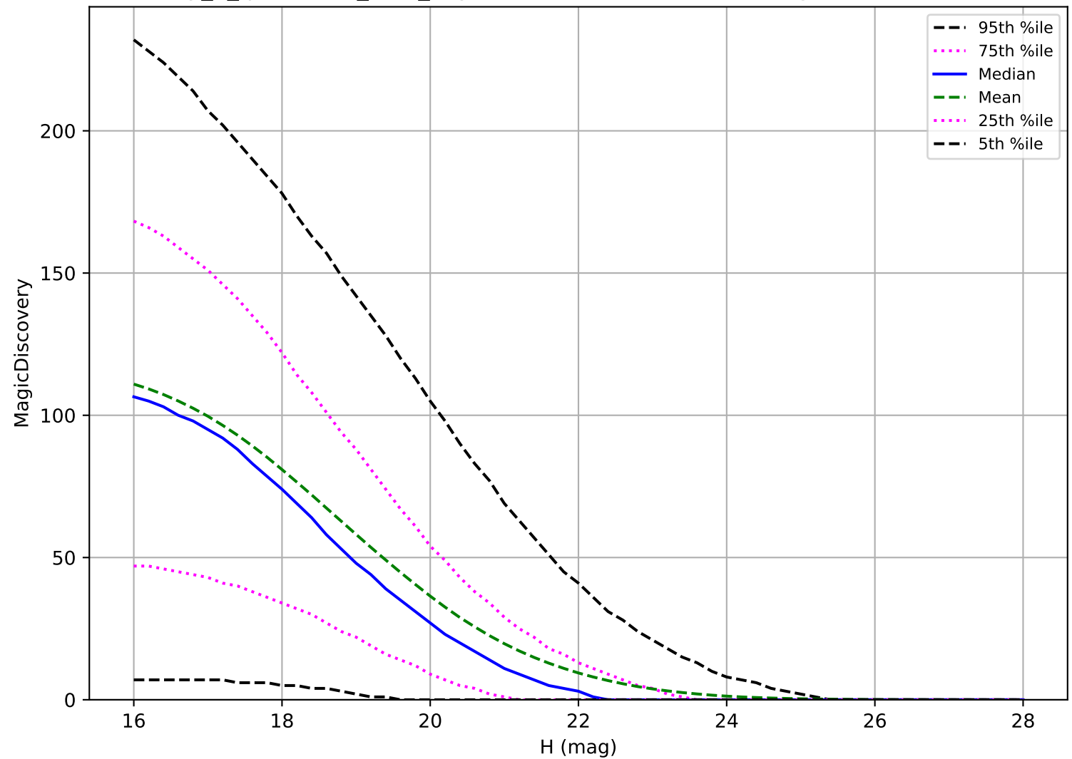
early_u_fpextra2.0_v3.4_10yrs: PHA 6 detections in 60 nights detection loss
