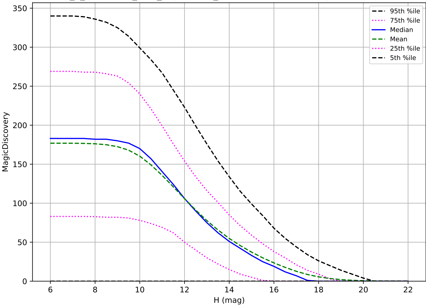
early_u_fpextra2.0_v3.4_10yrs: OCC_r5 6 detections in 60 nights detection loss
