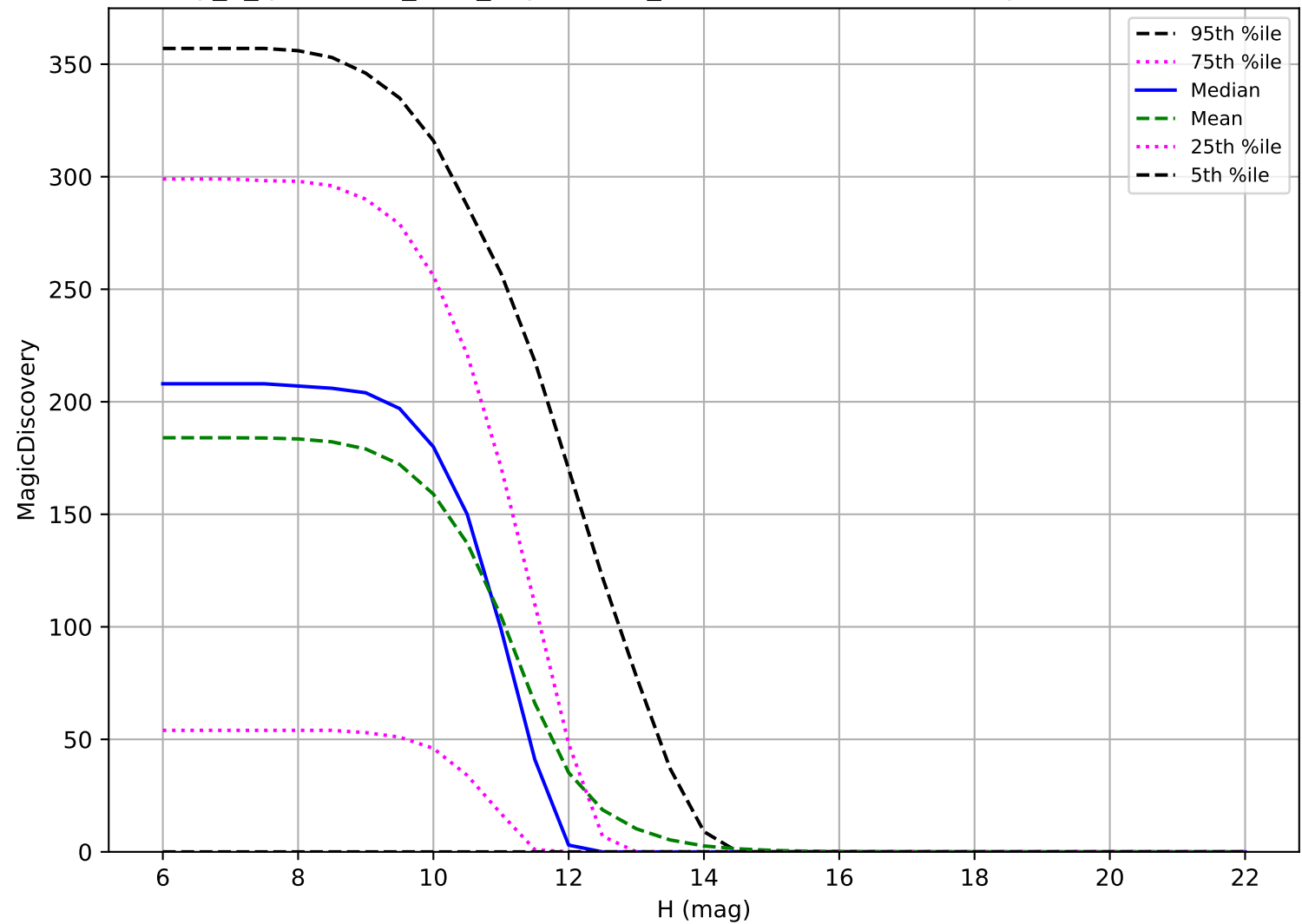
early_u_fpextra2.0_v3.4_10yrs: OCC_r20 6 detections in 60 nights detection loss
