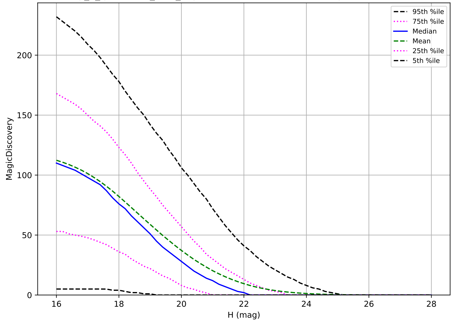
early_u_fpextra2.0_v3.4_10yrs: NEO 6 detections in 60 nights detection loss
