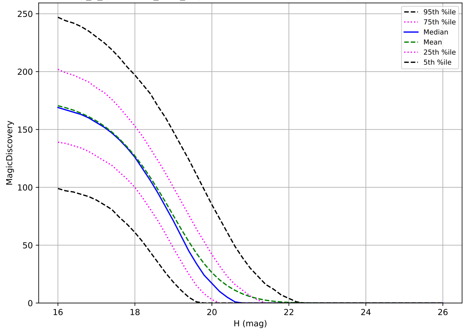
early_u_fpextra2.0_v3.4_10yrs: MBA 6 detections in 60 nights detection loss
