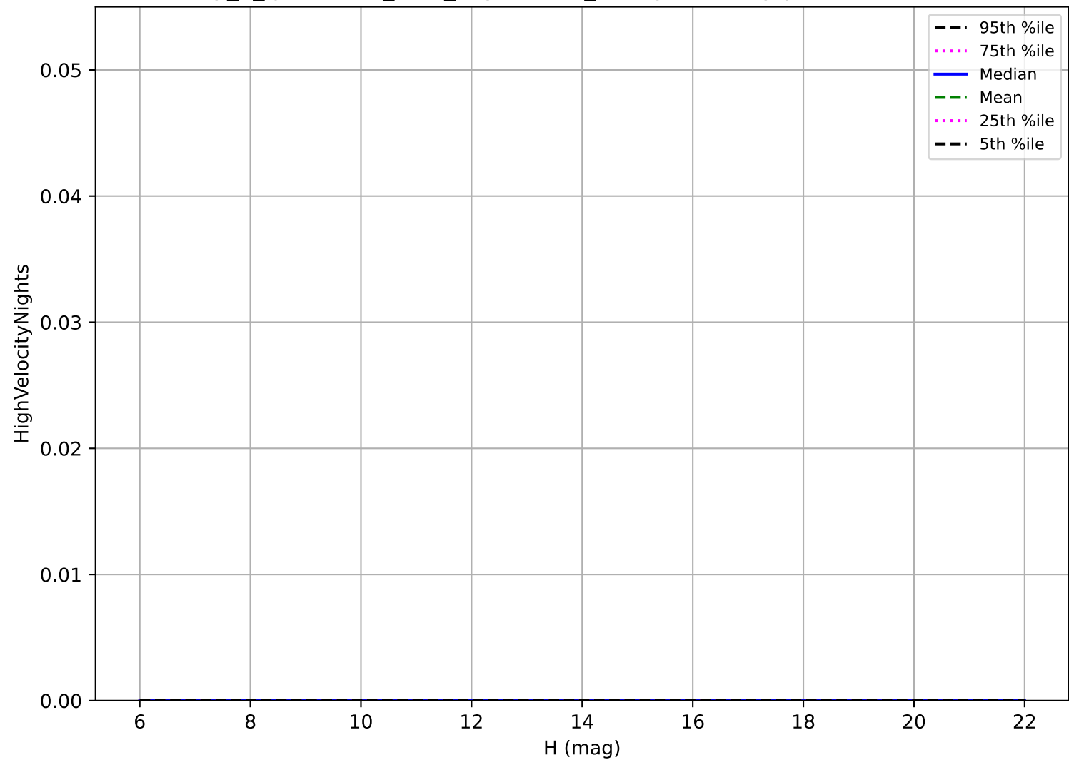
early_u_fpextra2.0_v3.4_10yrs: OCC_r5 High velocity pair detection loss
