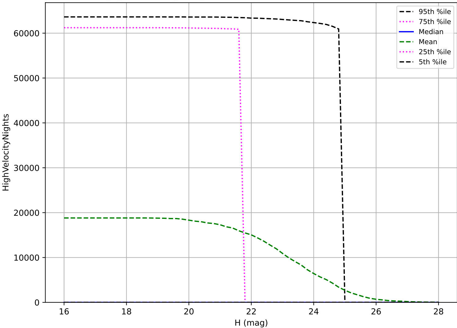
early_u_fpextra2.0_v3.4_10yrs: NEO High velocity pair detection loss
