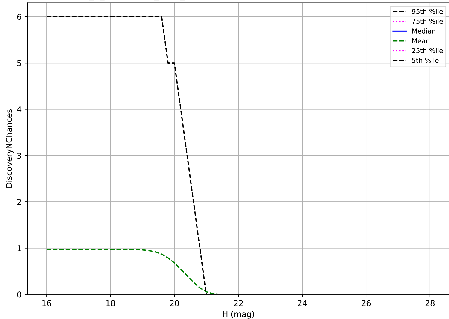
early_u_fpextra2.0_v3.4_10yrs: Vatira 3 pairs in 15 nights detection loss
