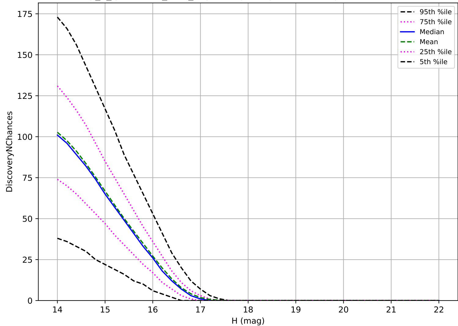
early_u_fpextra2.0_v3.4_10yrs: Trojan 3 pairs in 15 nights detection loss
