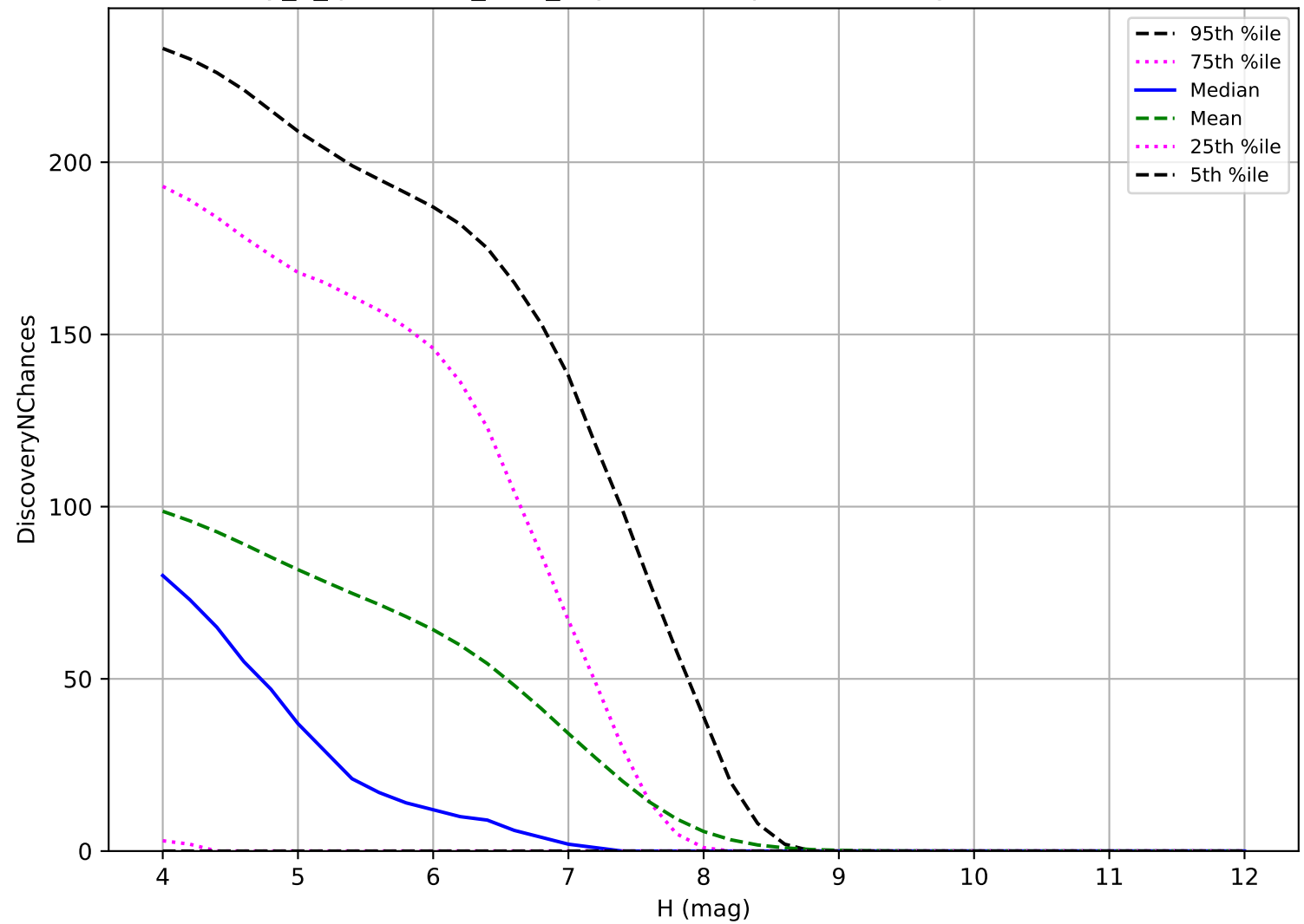
early_u_fpextra2.0_v3.4_10yrs: TNO 3 pairs in 15 nights detection loss
