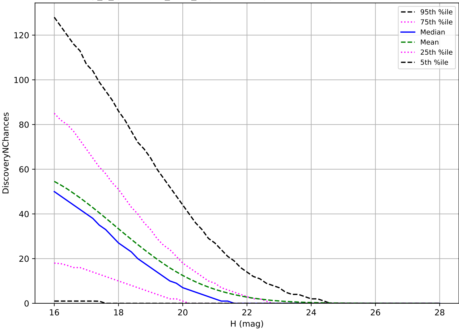
early_u_fpextra2.0_v3.4_10yrs: PHA 3 pairs in 15 nights detection loss
