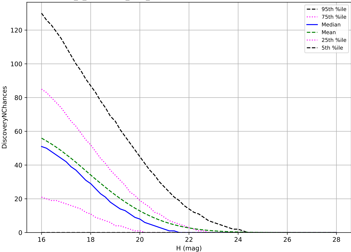
early_u_fpextra2.0_v3.4_10yrs: NEO 3 pairs in 15 nights detection loss
