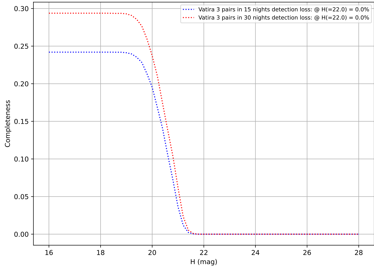
early_u_fpextra2.0_v3.4_10yrs: DifferentialCompleteness
