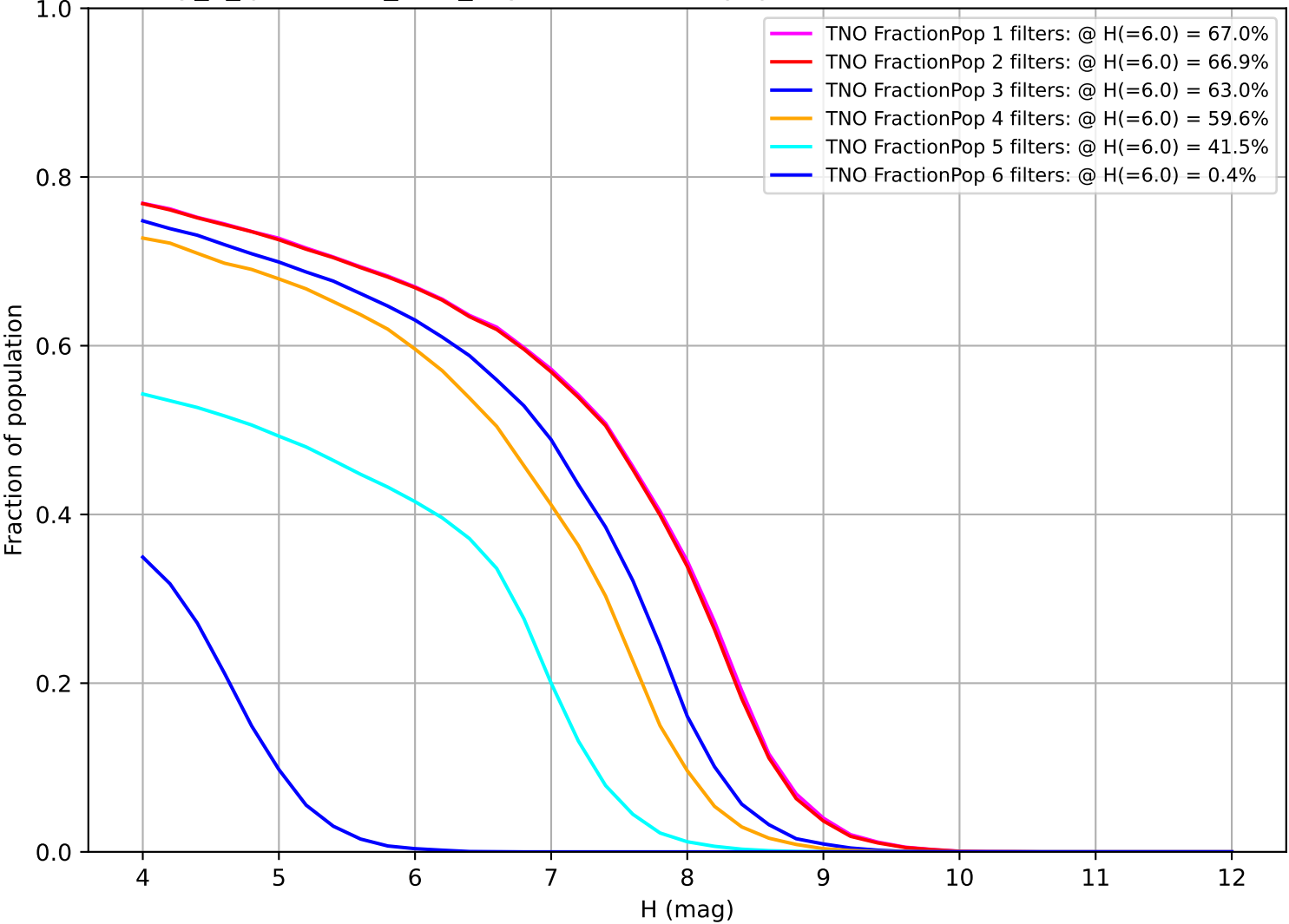
early_u_fpextra2.0_v3.4_10yrs: Fraction of population with colors in X filters TNO
