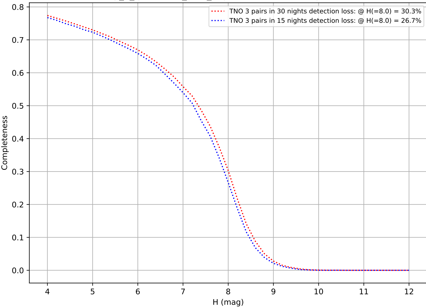
early_u_fpextra2.0_v3.4_10yrs: DifferentialCompleteness
