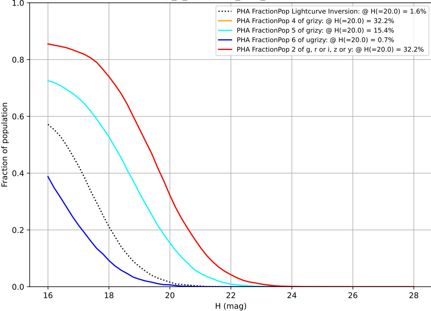
early_u_fpextra2.0_v3.4_10yrs PHA
