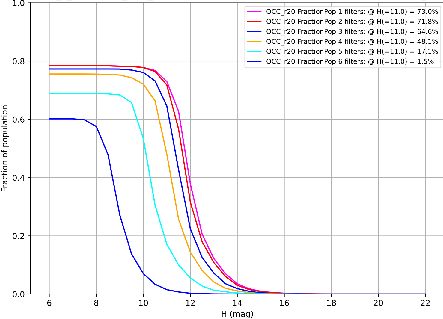
early_u_fpextra2.0_v3.4_10yrs: Fraction of population with colors in X filters OCC_r20
