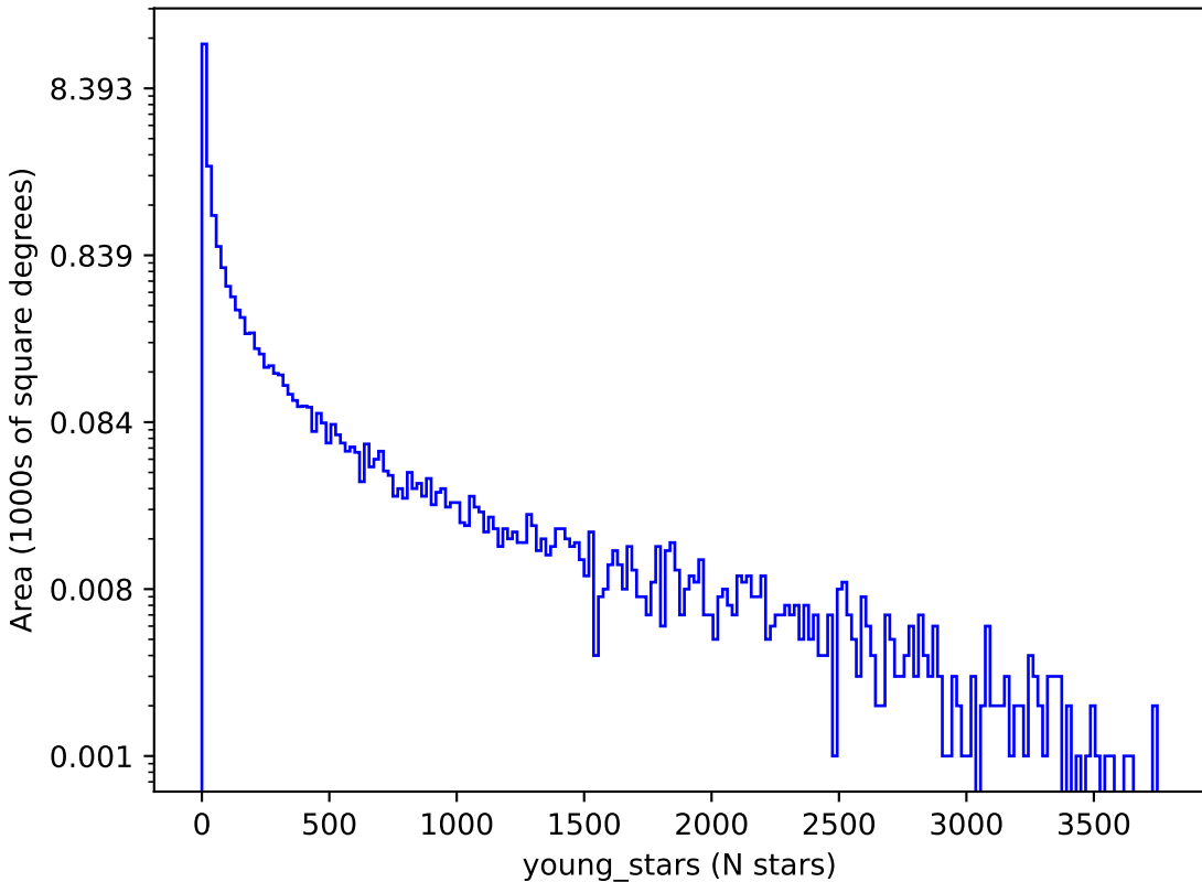
early_u_fpextra2.0_v3.4_10yrs : young_stars
