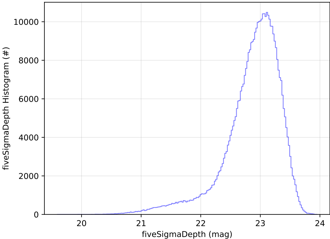
early_u_fpextra2.0_v3.4_10yrs z: fiveSigmaDepth Histogram
