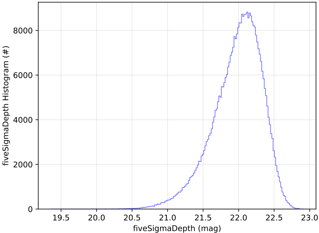
early_u_fpextra2.0_v3.4_10yrs y: fiveSigmaDepth Histogram
