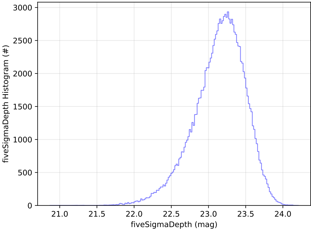
early_u_fpextra2.0_v3.4_10yrs u: fiveSigmaDepth Histogram
