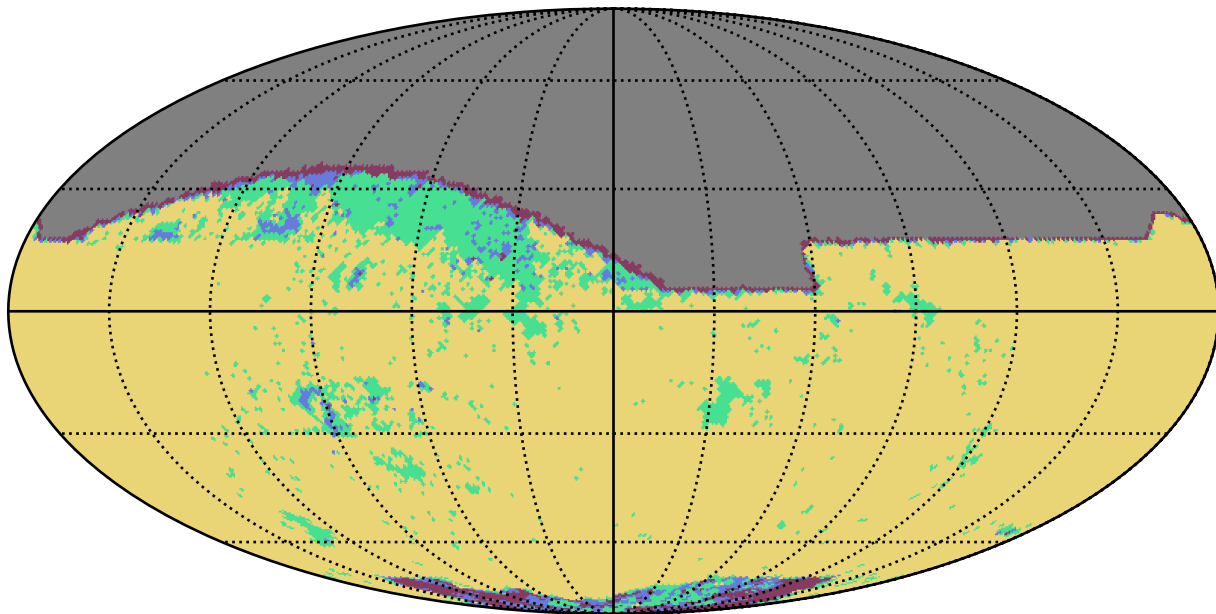
early_u_fpextra2.0_v3.4_10yrs z band: YearCoverage night
