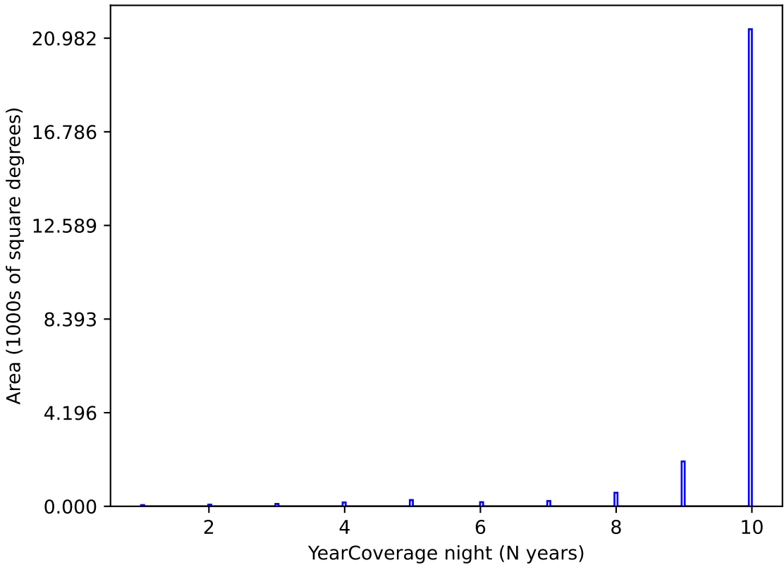
early_u_fpextra2.0_v3.4_10yrs y band: YearCoverage night
