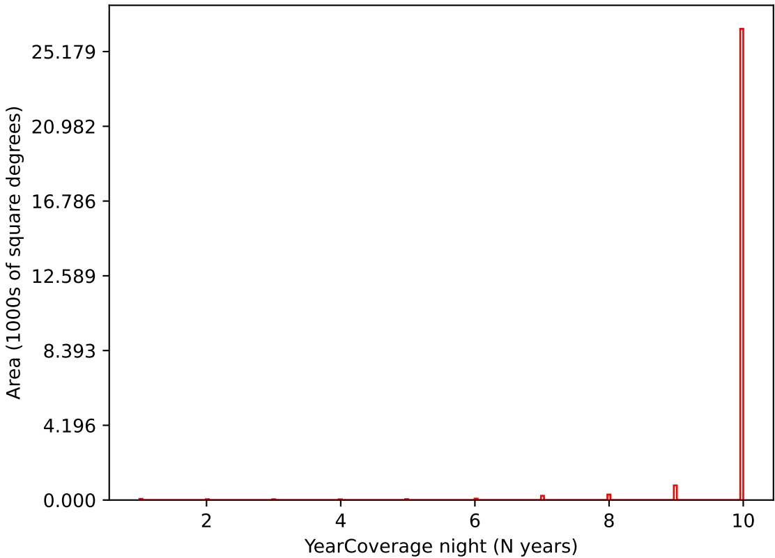
early_u_fpextra2.0_v3.4_10yrs i band: YearCoverage night
