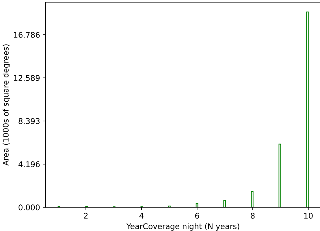
early_u_fpextra2.0_v3.4_10yrs g band: YearCoverage night
